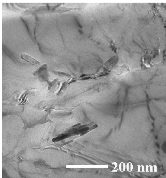
Fig. 3. Bright field TEM image of an Al-MWCNTs composite containing 1.0 wt.% of MWCNTs.
