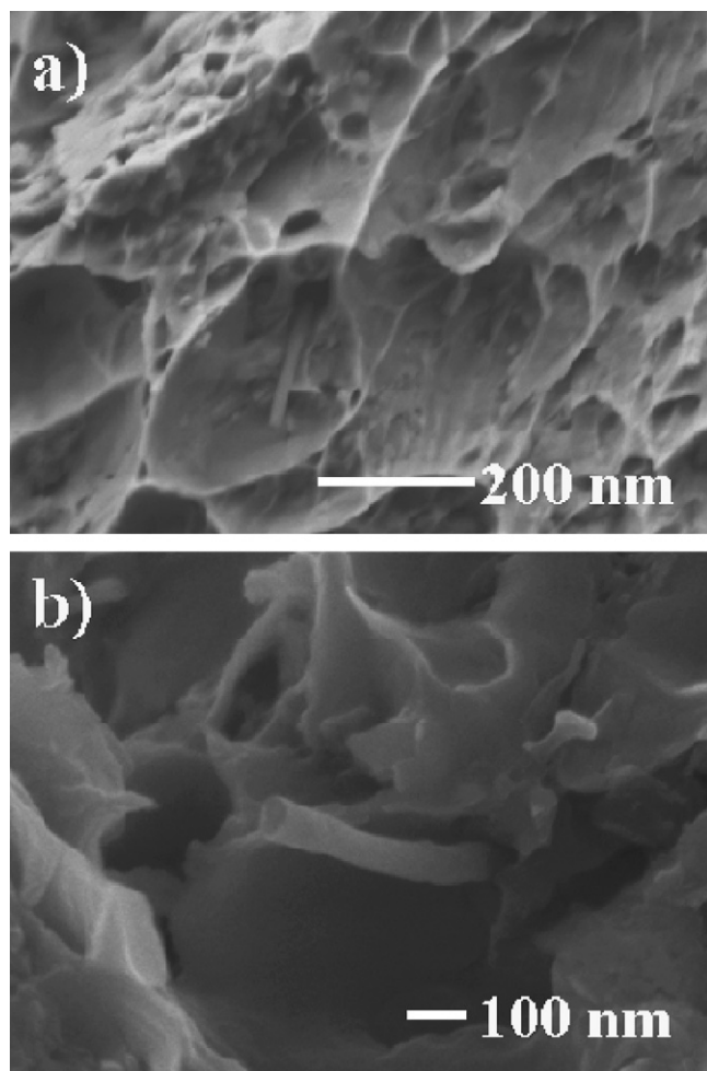
Fig. 4. Secondary electron SEM images on the broken surface showing CNTs outstanding from the broken Al-matrix surface. (a) Ductile fracture and (b) a CNT emerging from the broken surface.
