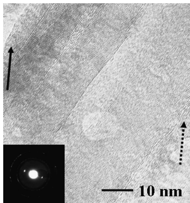
Fig. 5. HRTEM micrograph of the Al-MWCNTs composite showing the interface between MWCNTs and Al-matrix; the inset shows the corresponding diffraction pattern. The arrows show the transition layer between the MWCNTs core and the Al-matrix.
