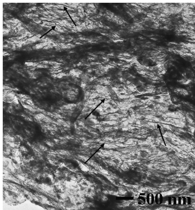
Fig. 2. Bright field TEM micrograph (low magnifications) of Al-MWCNTs composite containing 1.0 wt.% of MWCNTs, annealed for 3 h at 823 K in vacuum. The arrows indicate some MWCNTs.
