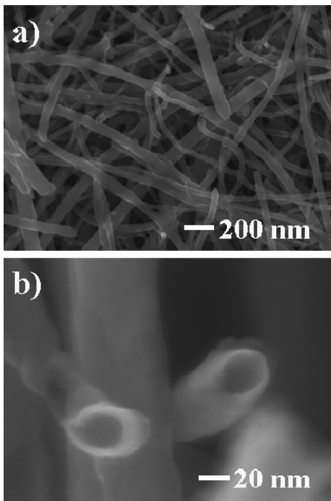
Fig. 1. Secondary electron SEM images from CNTs at (a) 40 and (b) 400 kX.
